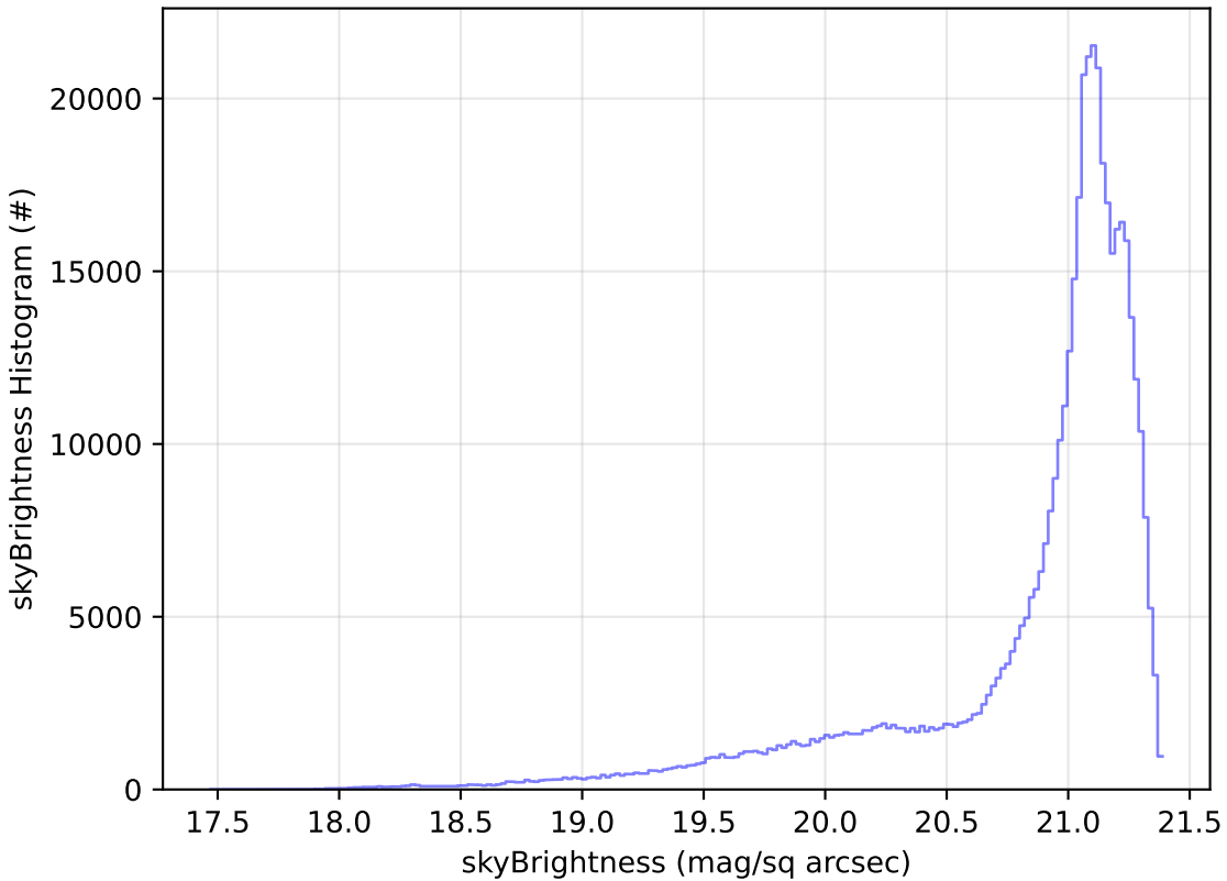
ddf_acor_sf25_lsf30_lsr10_v3.4_10yrs WFD r band: skyBrightness Histogram
