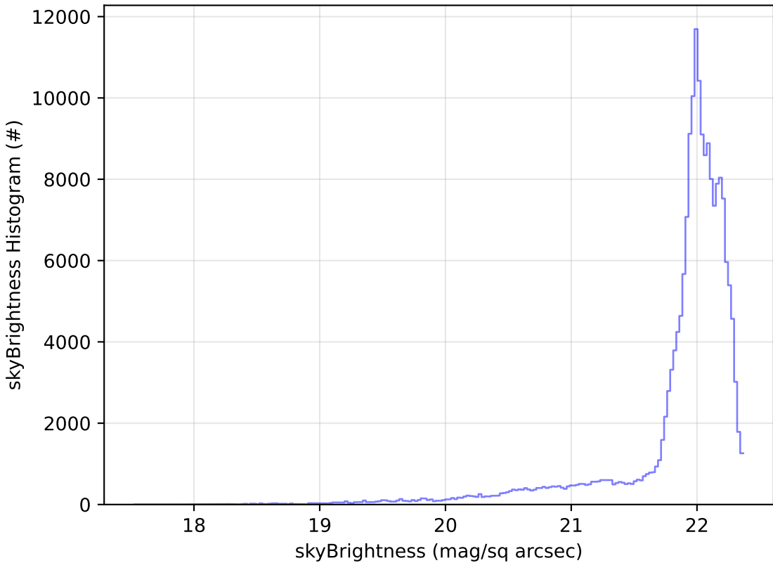
ddf_acor_sf25_lsf30_lsr10_v3.4_10yrs WFD g band: skyBrightness Histogram
