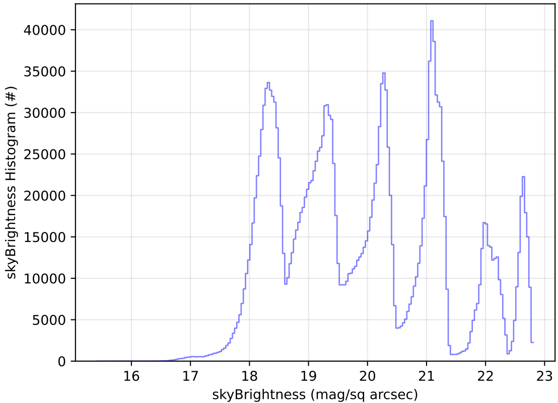
ddf_acor_sf25_lsf30_lsr10_v3.4_10yrs WFD all bands: skyBrightness Histogram
