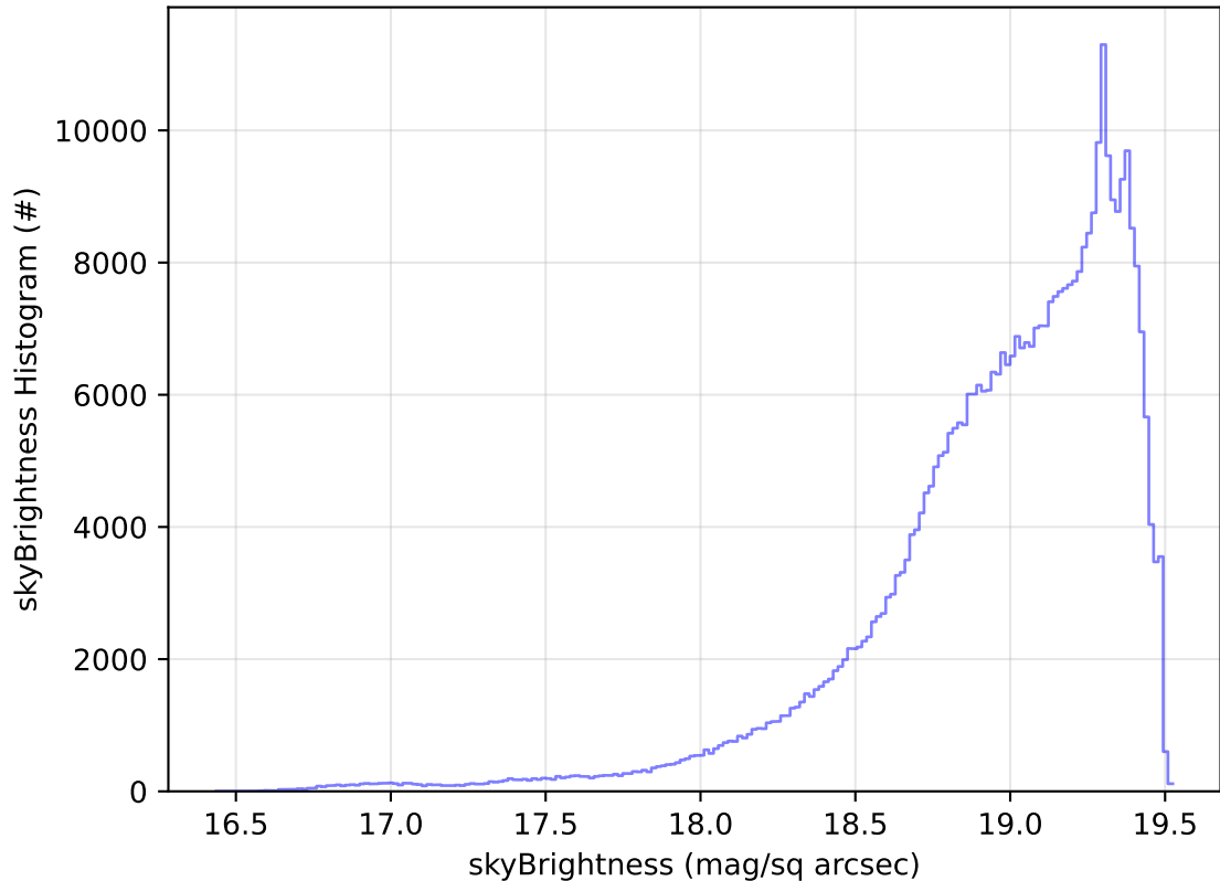
ddf_acor_sf25_lsf30_lsr10_v3.4_10yrs All sky z band: skyBrightness Histogram
