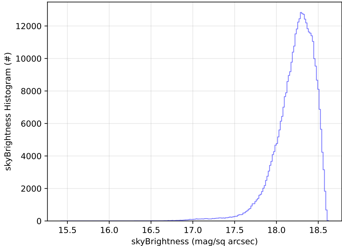
ddf_acor_sf25_lsf30_lsr10_v3.4_10yrs All sky y band: skyBrightness Histogram
