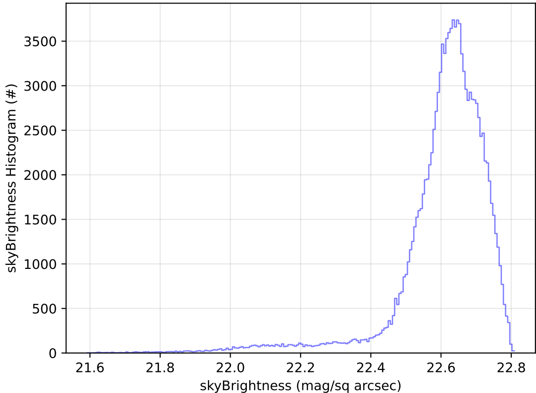
ddf_acor_sf25_lsf30_lsr10_v3.4_10yrs All sky u band: skyBrightness Histogram
