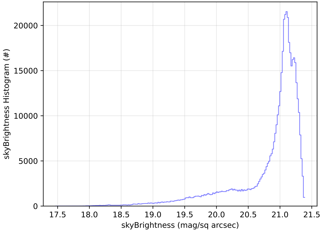
ddf_acor_sf25_lsf30_lsr10_v3.4_10yrs All sky r band: skyBrightness Histogram
