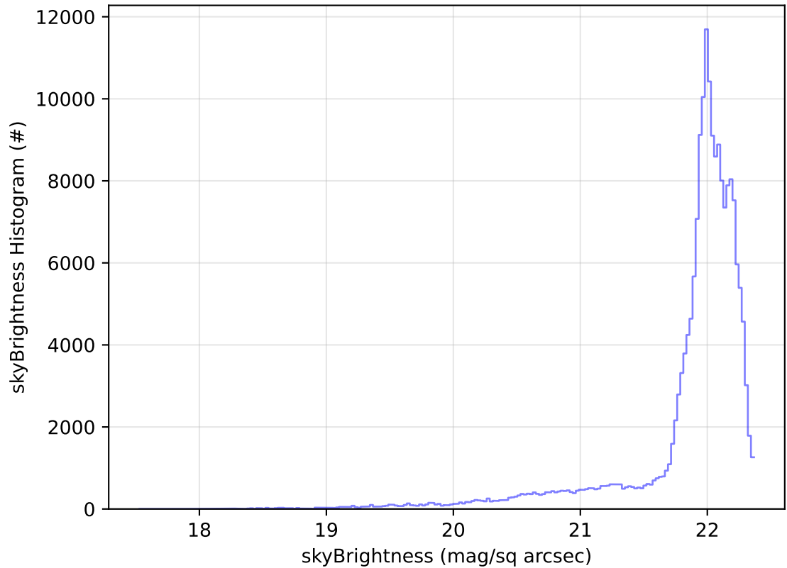
ddf_acor_sf25_lsf30_lsr10_v3.4_10yrs All sky g band: skyBrightness Histogram
