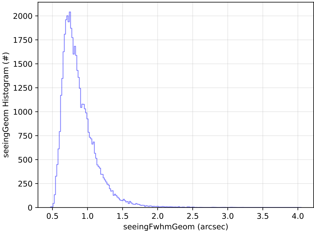
ddf_acor_sf25_lsf30_lsr10_v3.4_10yrs Yr 1 z band: seeingGeom Histogram
