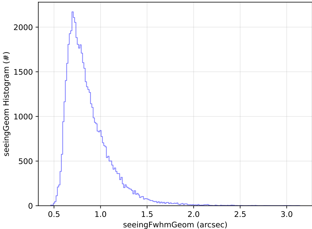
ddf_acor_sf25_lsf30_lsr10_v3.4_10yrs Yr 1 i band: seeingGeom Histogram
