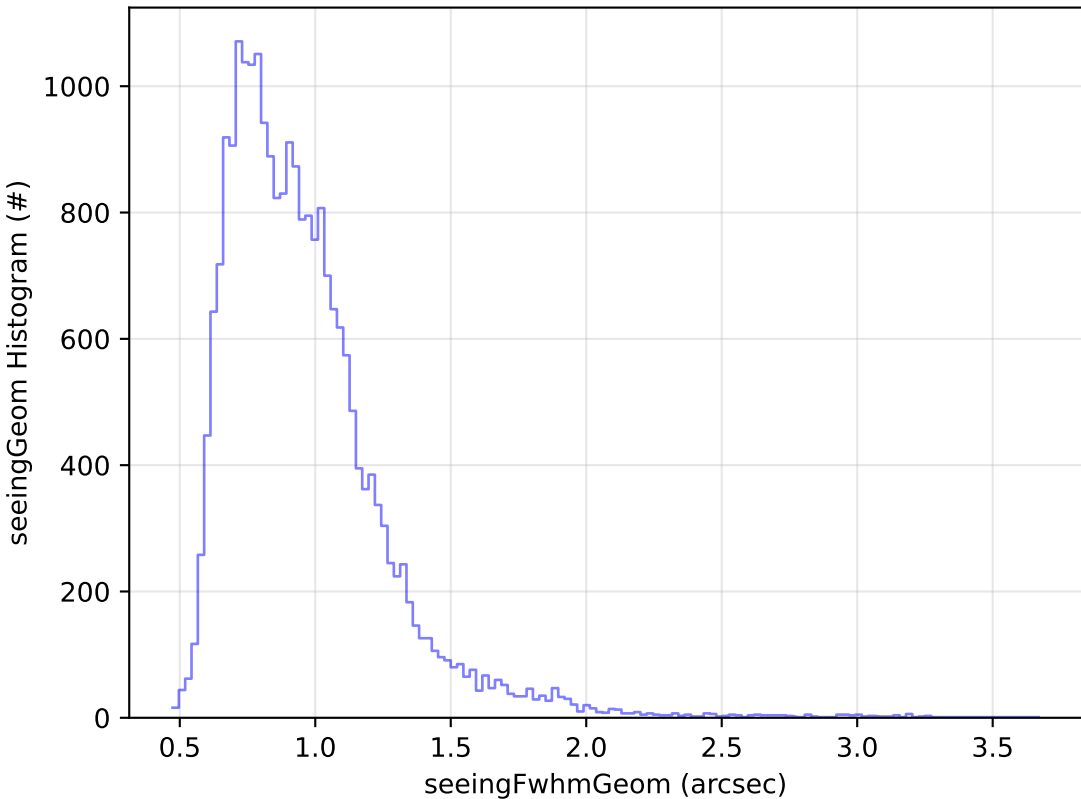
ddf_acor_sf25_lsf30_lsr10_v3.4_10yrs Yr 1 g band: seeingGeom Histogram
