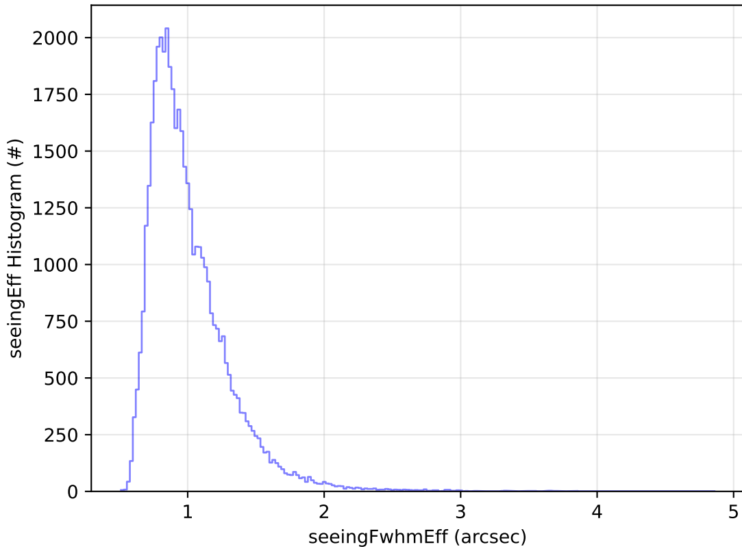
ddf_acor_sf25_lsf30_lsr10_v3.4_10yrs Yr 1 z band: seeingEff Histogram
