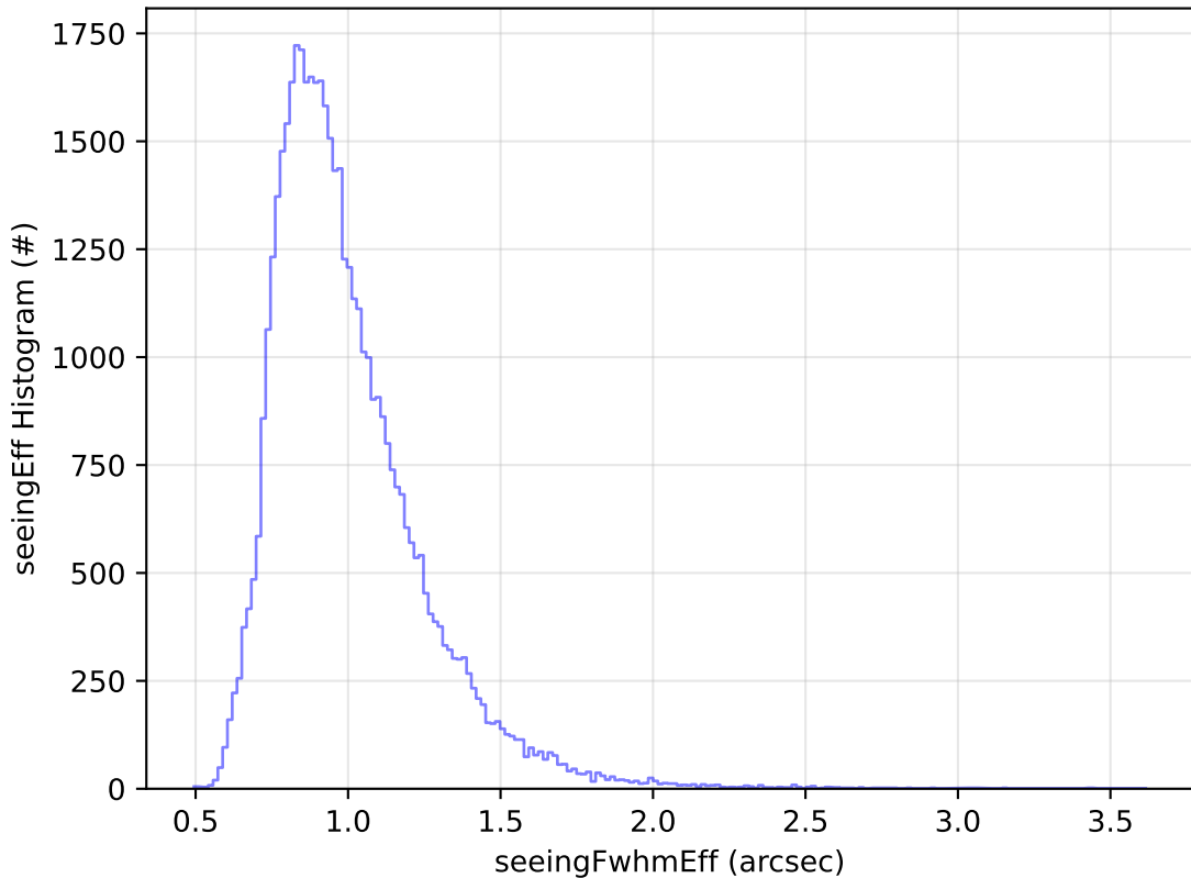
ddf_acor_sf25_lsf30_lsr10_v3.4_10yrs Yr 1 y band: seeingEff Histogram
