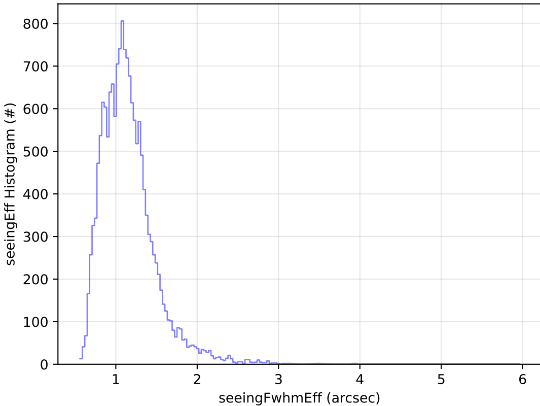
ddf_acor_sf25_lsf30_lsr10_v3.4_10yrs Yr 1 u band: seeingEff Histogram
