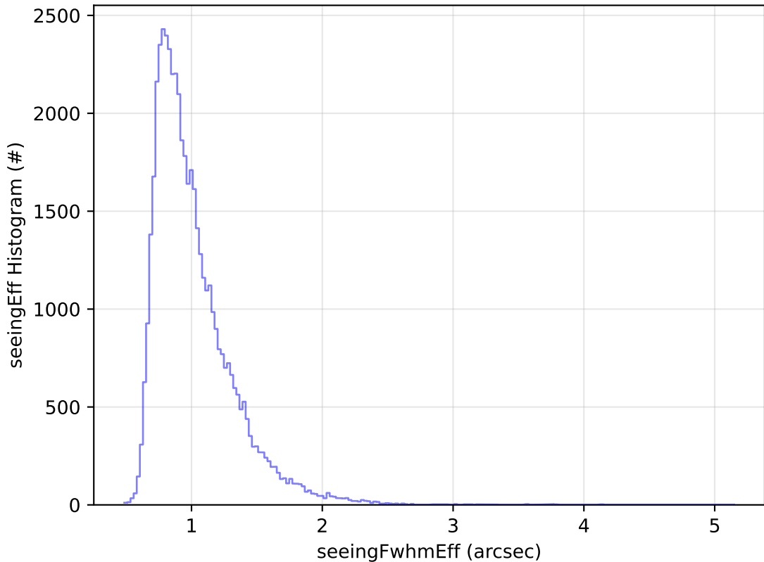
ddf_acor_sf25_lsf30_lsr10_v3.4_10yrs Yr 1 r band: seeingEff Histogram
