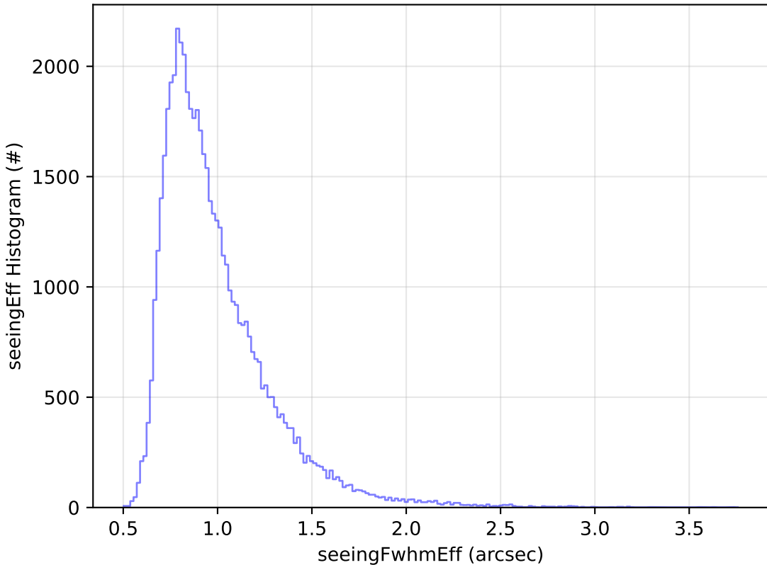
ddf_acor_sf25_lsf30_lsr10_v3.4_10yrs Yr 1 i band: seeingEff Histogram
