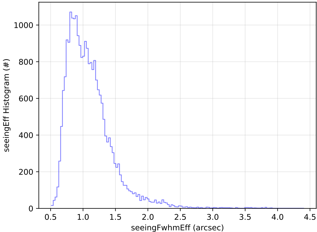
ddf_acor_sf25_lsf30_lsr10_v3.4_10yrs Yr 1 g band: seeingEff Histogram
