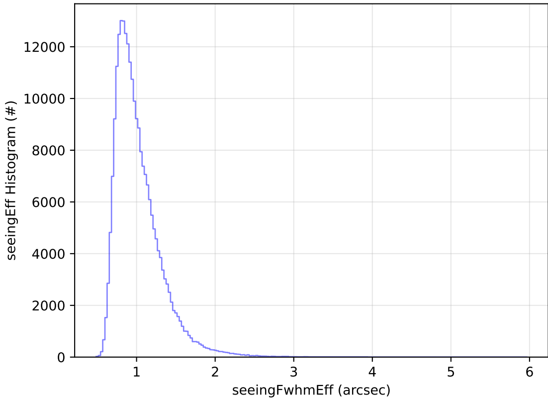
ddf_acor_sf25_Isf30_Isr10_v3.4_10yrs Yr 1 all bands: seeingEff Histogram
