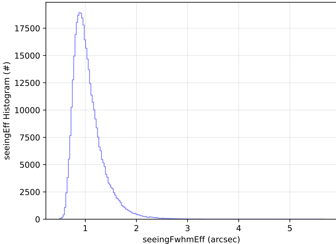
ddf_acor_sf25_lsf30_lsr10_v3.4_10yrs WFD y band: seeingEff Histogram
