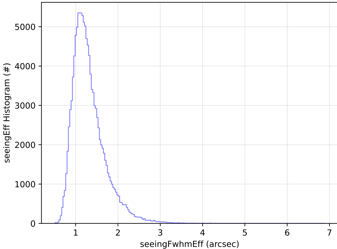
ddf_acor_sf25_lsf30_lsr10_v3.4_10yrs WFD u band: seeingEff Histogram
