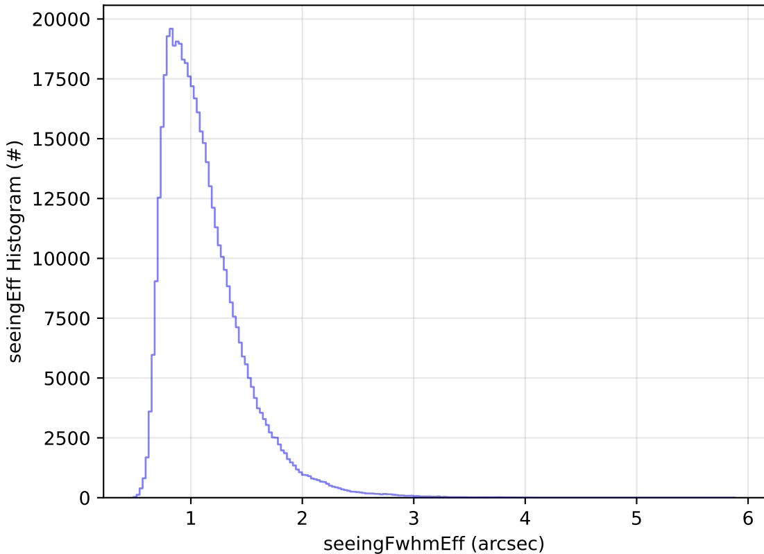
ddf_acor_sf25_lsf30_lsr10_v3.4_10yrs WFD r band: seeingEff Histogram
