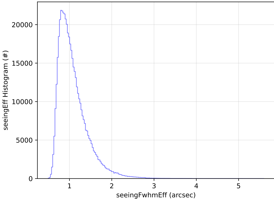
ddf_acor_sf25_lsf30_lsr10_v3.4_10yrs WFD i band: seeingEff Histogram
