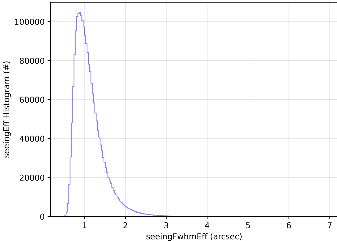
ddf_acor_sf25_lsf30_lsr10_v3.4_10yrs WFD all bands: seeingEff Histogram
