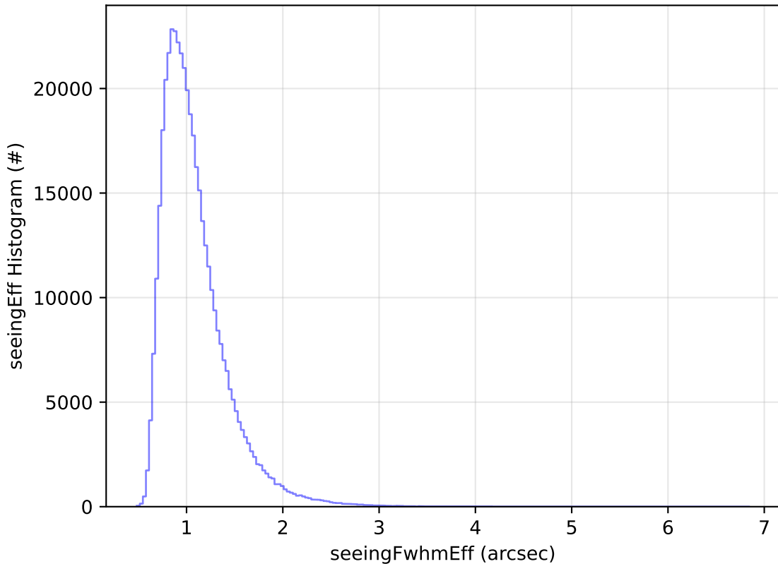
ddf_acor_sf25_lsf30_lsr10_v3.4_10yrs All sky z band: seeingEff Histogram
