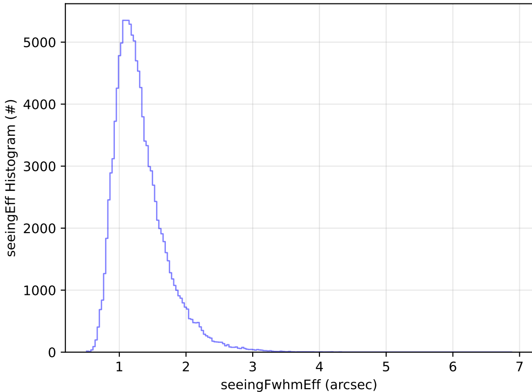
ddf_acor_sf25_lsf30_lsr10_v3.4_10yrs All sky u band: seeingEff Histogram
