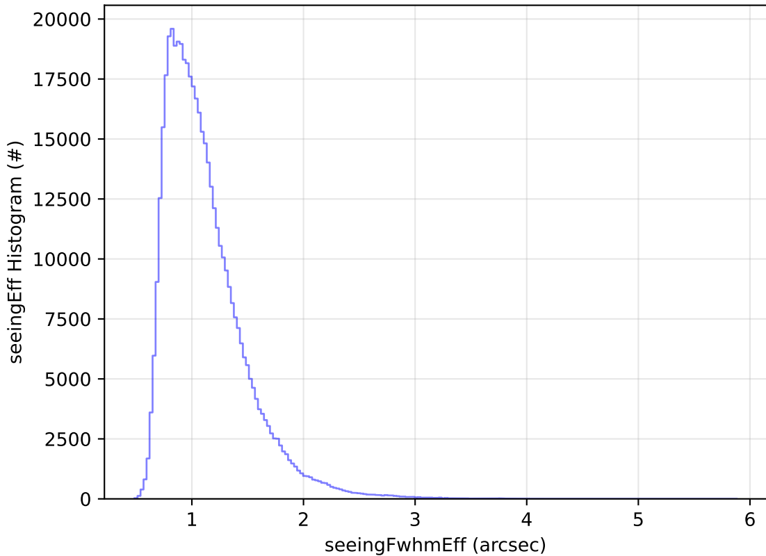
ddf_acor_sf25_lsf30_lsr10_v3.4_10yrs All sky r band: seeingEff Histogram
