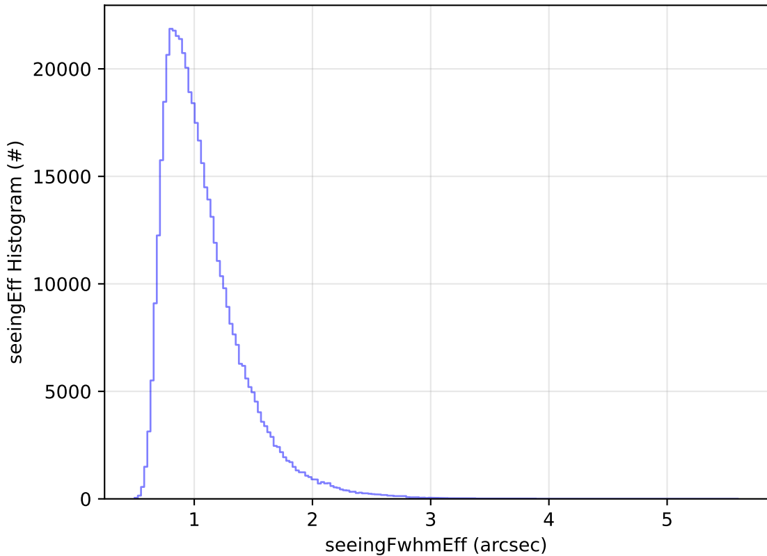
ddf_acor_sf25_lsf30_lsr10_v3.4_10yrs All sky i band: seeingEff Histogram
