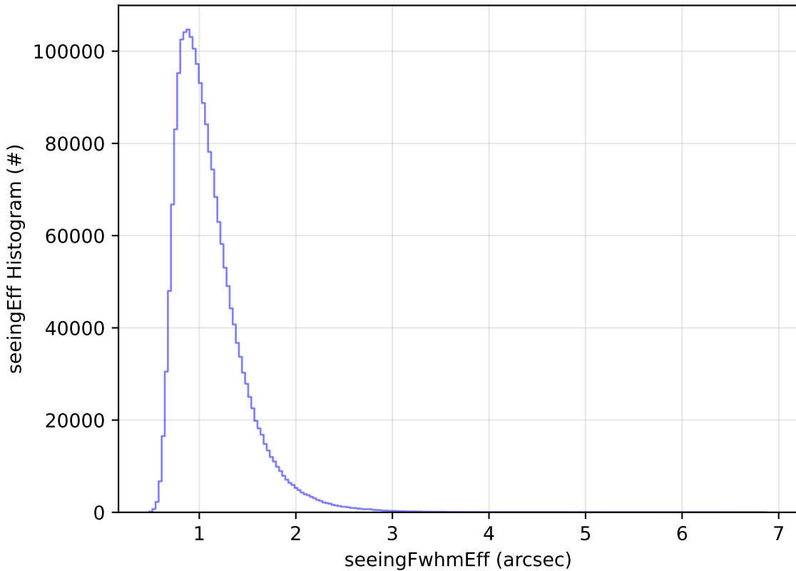
ddf_acor_sf25_lsf30_lsr10_v3.4_10yrs All sky all bands: seeingEff Histogram
