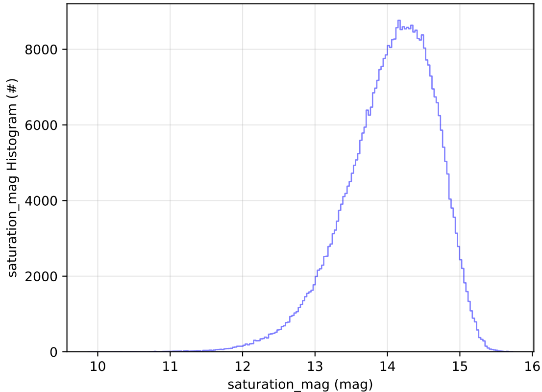
ddf_acor_sf25_lsf30_lsr10_v3.4_10yrs WFD z band: saturation_mag Histogram
