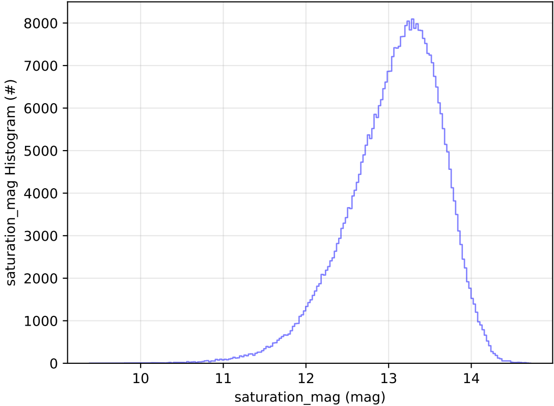
ddf_acor_sf25_lsf30_lsr10_v3.4_10yrs WFD y band: saturation_mag Histogram
