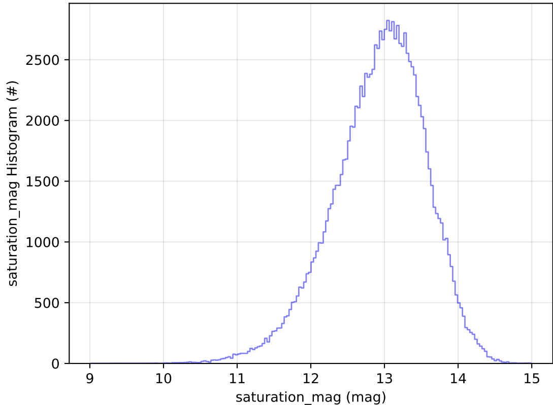
ddf_acor_sf25_lsf30_lsr10_v3.4_10yrs WFD u band: saturation_mag Histogram
