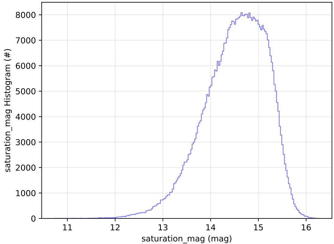
ddf_acor_sf25_lsf30_lsr10_v3.4_10yrs WFD r band: saturation_mag Histogram
