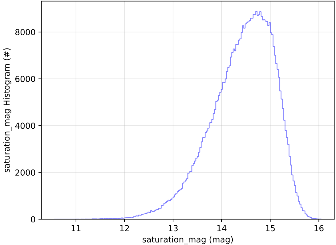
ddf_acor_sf25_lsf30_lsr10_v3.4_10yrs WFD i band: saturation_mag Histogram
