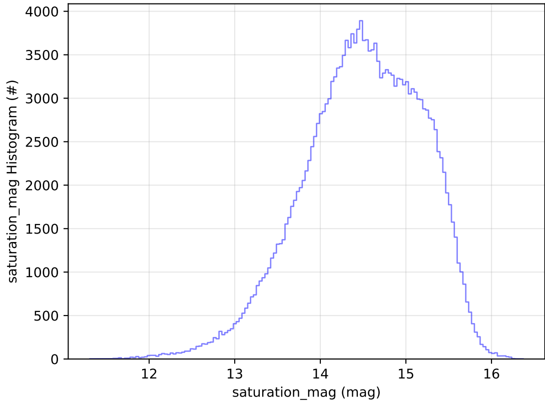
ddf_acor_sf25_lsf30_lsr10_v3.4_10yrs WFD g band: saturation_mag Histogram
