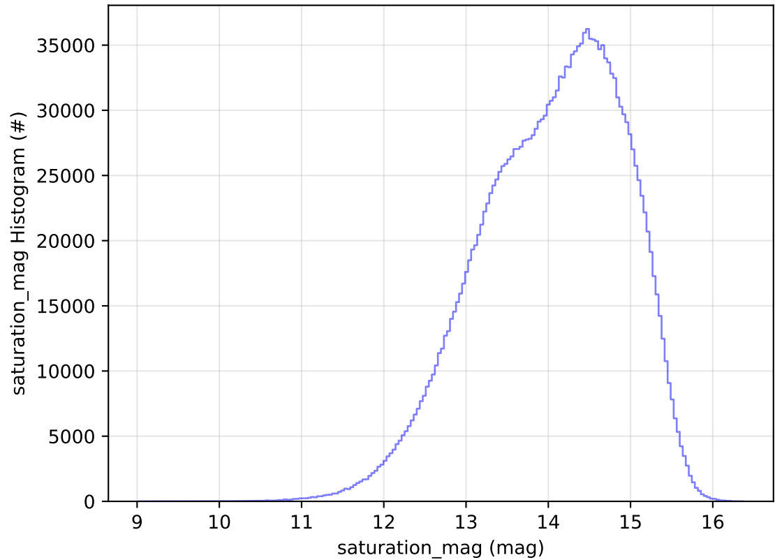
ddf_acor_sf25_lsf30_lsr10_v3.4_10yrs WFD all bands: saturation_mag Histogram
