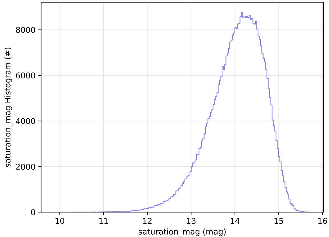
ddf_acor_sf25_lsf30_lsr10_v3.4_10yrs All sky z band: saturation_mag Histogram
