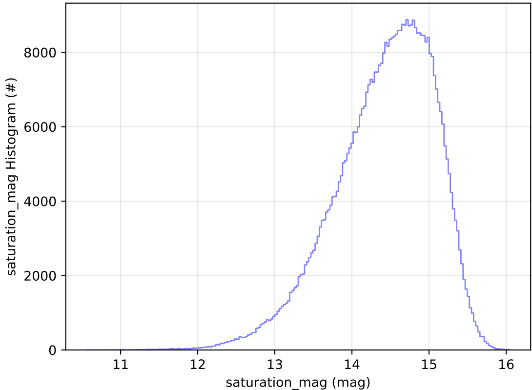
ddf_acor_sf25_lsf30_lsr10_v3.4_10yrs All sky i band: saturation_mag Histogram
