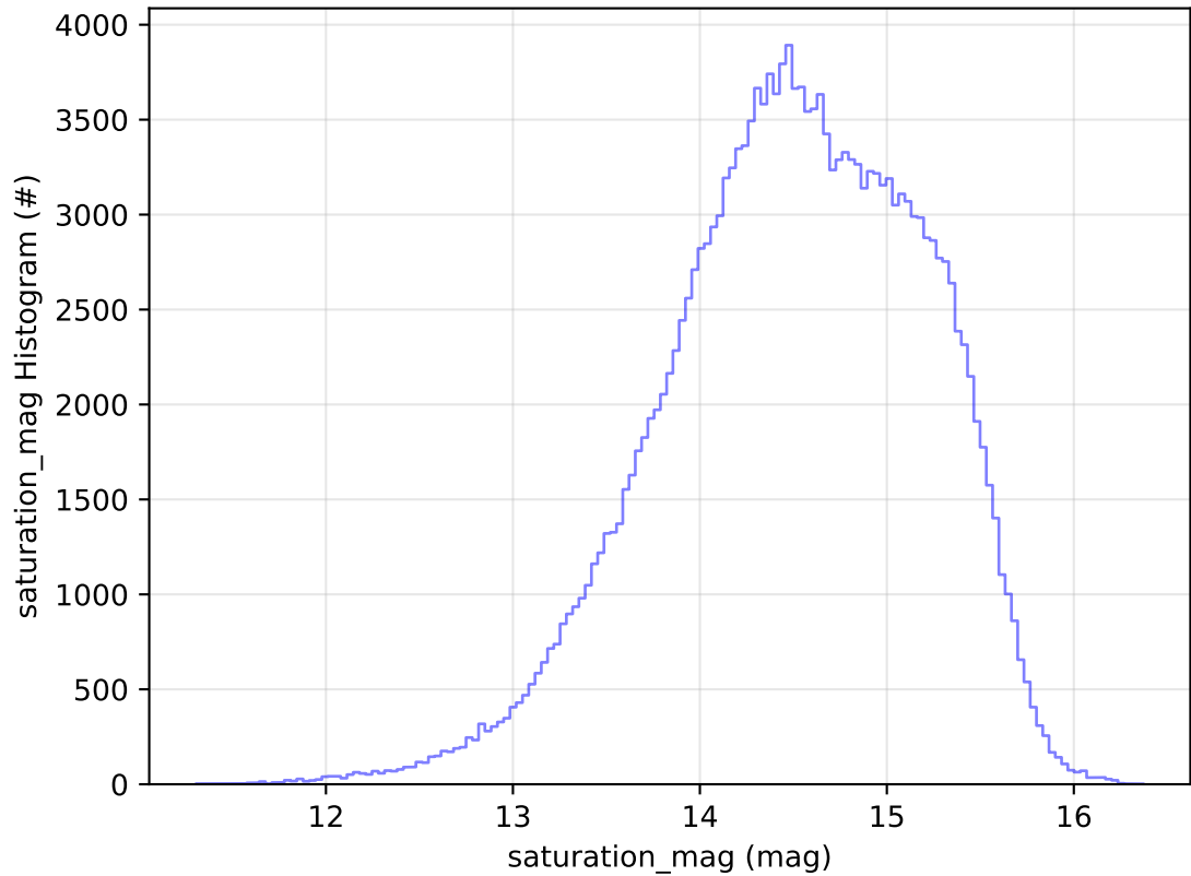
ddf_acor_sf25_lsf30_lsr10_v3.4_10yrs All sky g band: saturation_mag Histogram
