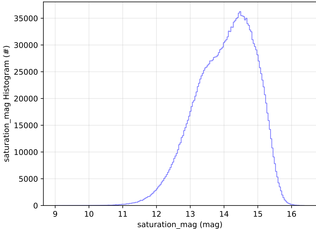
ddf_acor_sf25_lsf30_lsr10_v3.4_10yrs All sky all bands: saturation_mag Histogram
