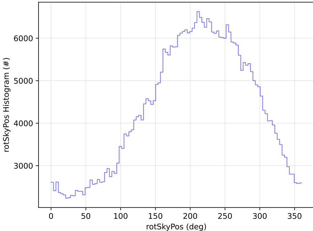
ddf_acor_sf25_lsf30_lsr10_v3.4_10yrs WFD z band: rotSkyPos Histogram
