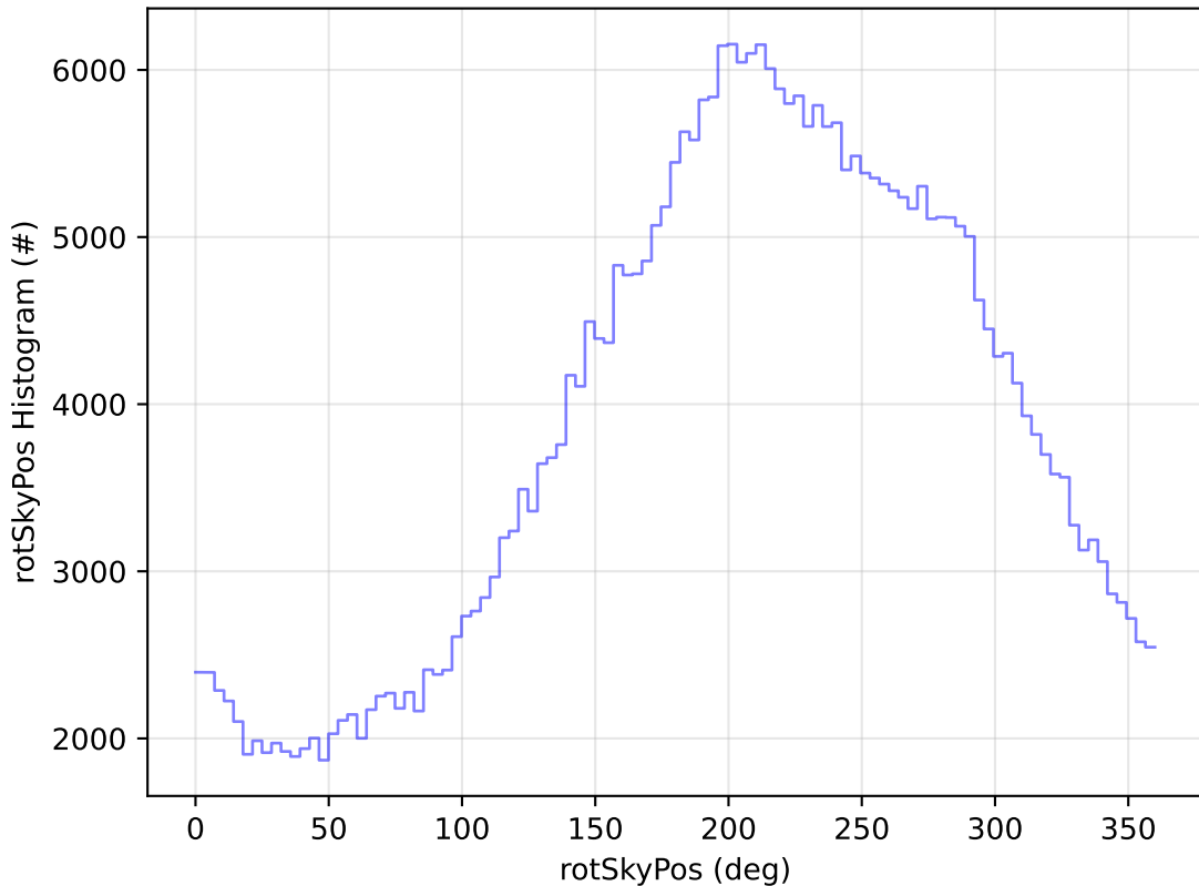
ddf_acor_sf25_lsf30_lsr10_v3.4_10yrs WFD y band: rotSkyPos Histogram
