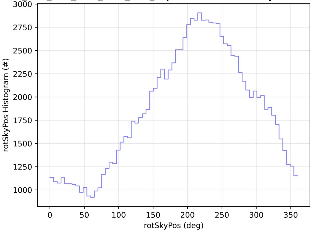
ddf_acor_sf25_lsf30_lsr10_v3.4_10yrs WFD u band: rotSkyPos Histogram
