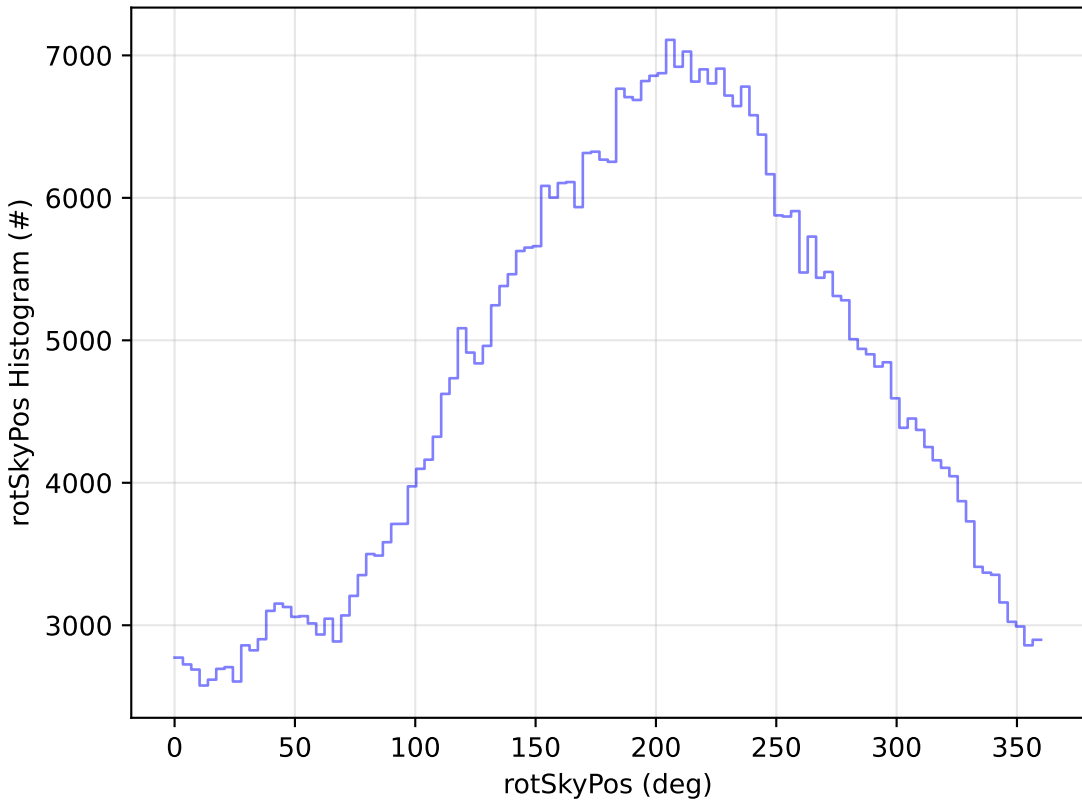
ddf_acor_sf25_lsf30_lsr10_v3.4_10yrs WFD r band: rotSkyPos Histogram
