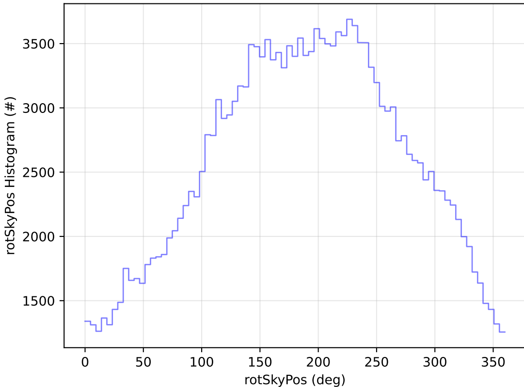
ddf_acor_sf25_lsf30_lsr10_v3.4_10yrs WFD g band: rotSkyPos Histogram
