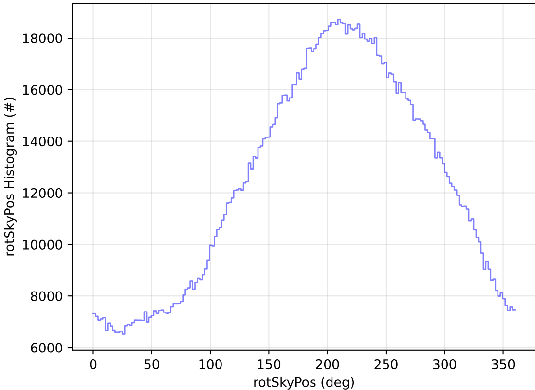
ddf_acor_sf25_lsf30_lsr10_v3.4_10yrs WFD all bands: rotSkyPos Histogram
