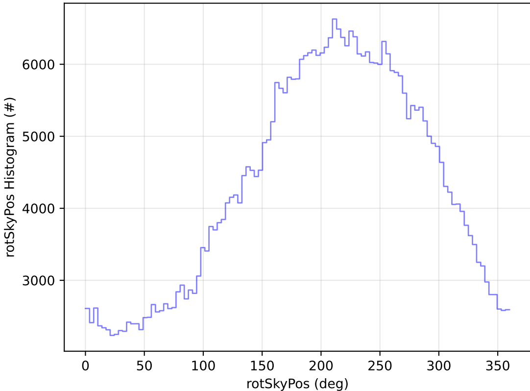
ddf_acor_sf25_lsf30_lsr10_v3.4_10yrs All sky z band: rotSkyPos Histogram
