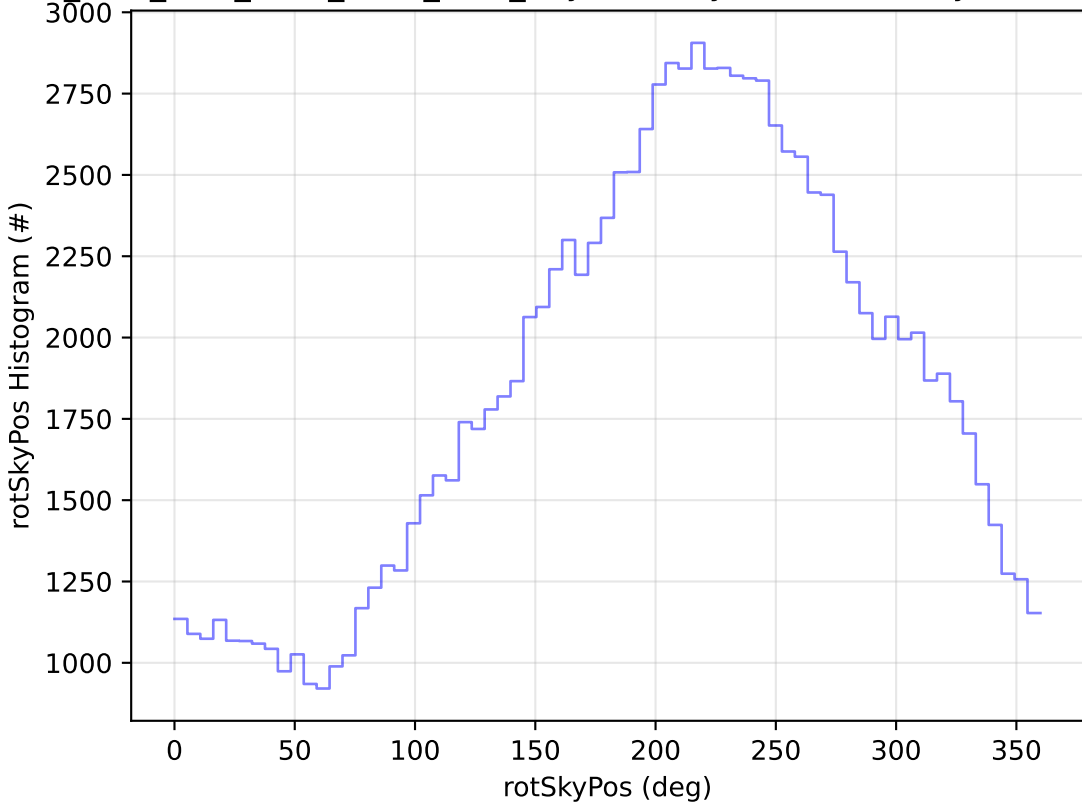
ddf_acor_sf25_lsf30_lsr10_v3.4_10yrs All sky u band: rotSkyPos Histogram
