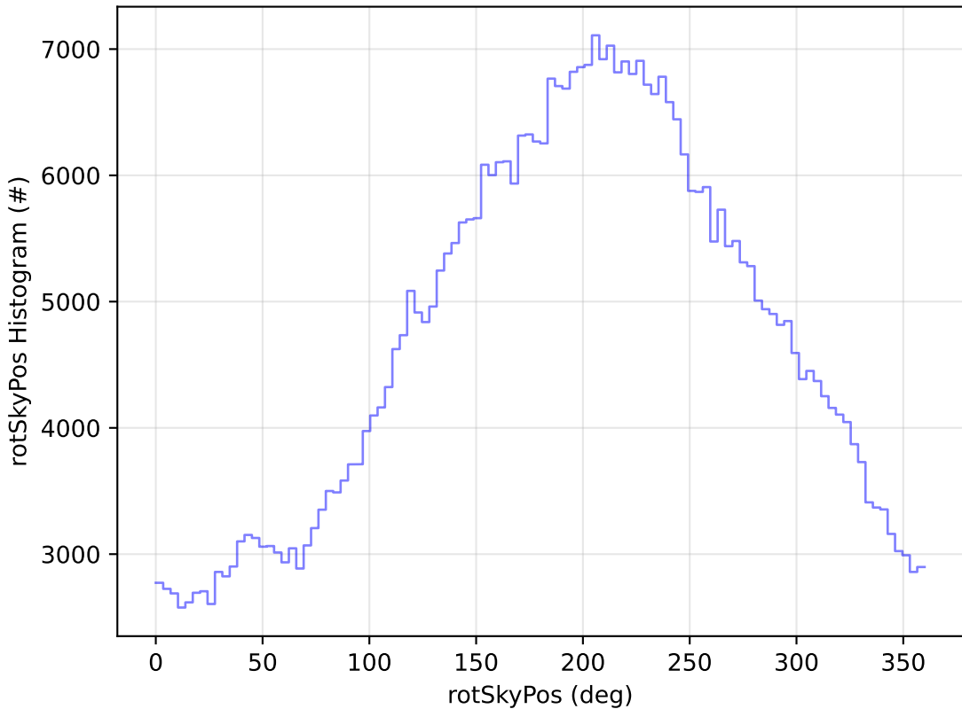
ddf_acor_sf25_lsf30_lsr10_v3.4_10yrs All sky r band: rotSkyPos Histogram
