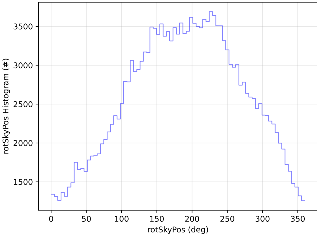
ddf_acor_sf25_lsf30_lsr10_v3.4_10yrs All sky g band: rotSkyPos Histogram
