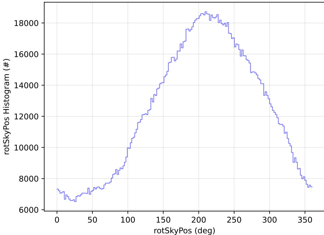
ddf_acor_sf25_lsf30_lsr10_v3.4_10yrs All sky all bands: rotSkyPos Histogram
